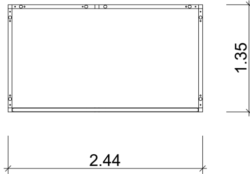
RSAL-120002 Podest lang (2440x1350), Stahl komplett
